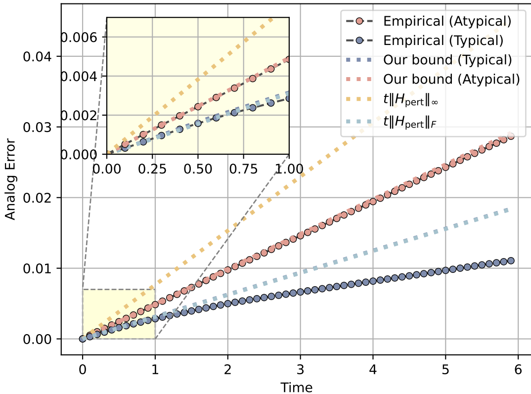
2D-lattice QIMF, long-time evolution with disorder
